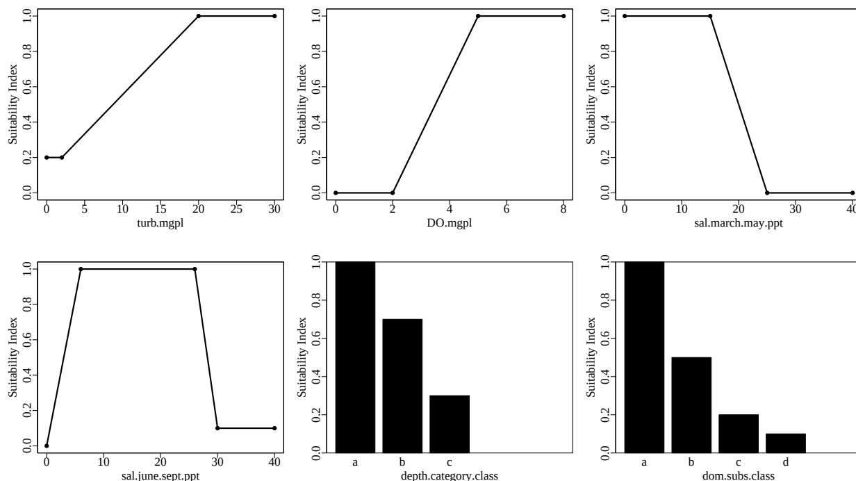
Figure 1. Suitability index graphs for variables included in the atlanticcroakerOtherTideLt0.5m model in ecorest.
